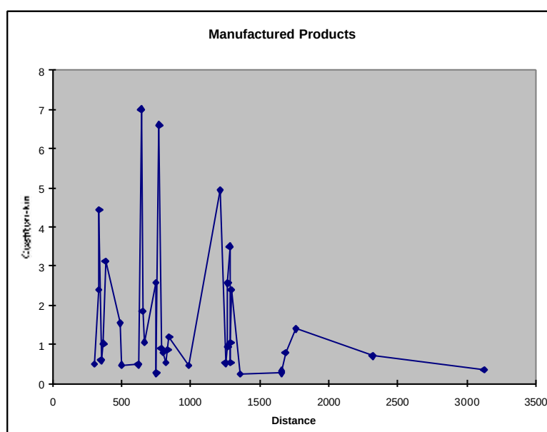
Figure 4.1: Relationship between cost per tonkm and distance for manufactured products as established in a Danish survey.
